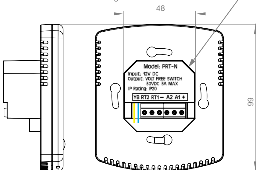
Wiring Detail
