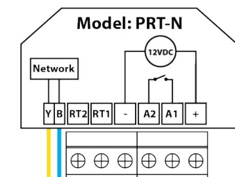
Wiring Detail
